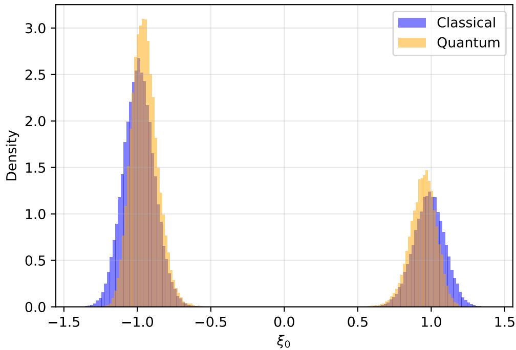
Distribution of Centroid Mode ( \xi_0 )
